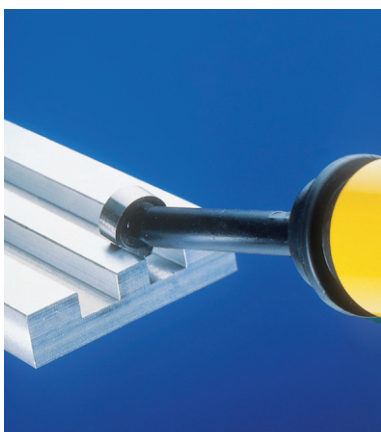
GT-KEYWAY-BURR - For deburring narrow or wide slots. Internal and external keyways. EL1400GT
