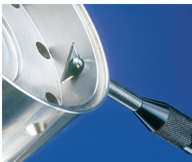
LARGE REVERSIBLE COUNTERSINK RC2200GT Patented
