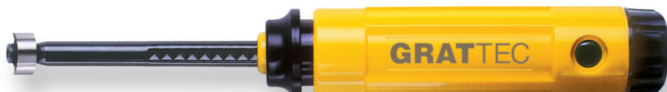
GT-KEYWAY-BURR - For deburring narrow or wide slots. Internal and external keyways. EL1400GT
